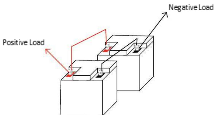
Figure 3: Two BB5012 Batteries connected in Parallel to create a 12V 100Ah Battery Bank
