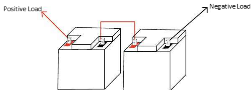
Figure 4: Two BB5012 Batteries Connected in Series to create a 24V 50Ah Battery Bank
